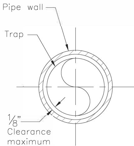
CROSS SECTION OF MH OUT PIPE WITH TRAP INSTALLED
