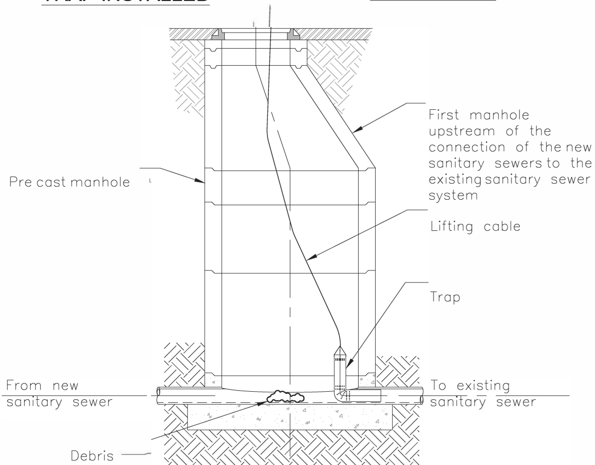
CUSTOM FABRICATED METAL TRAP
