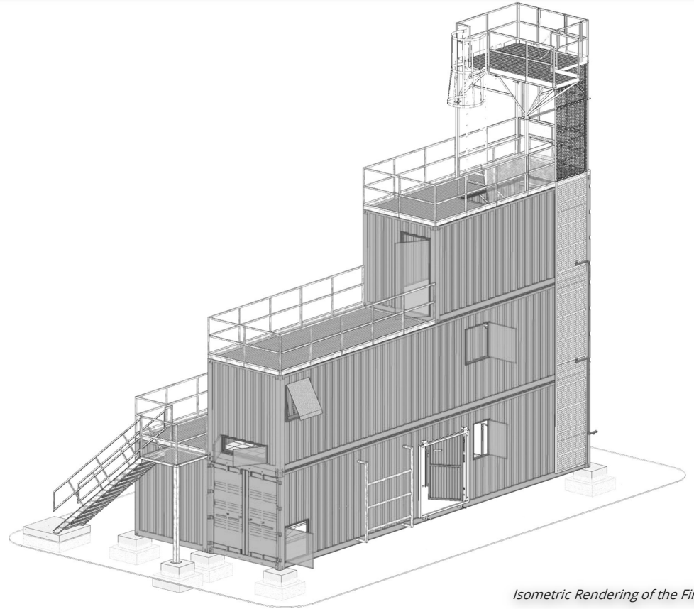
Architectural renderings of the Fire Rescue Training Facility and Tower.
